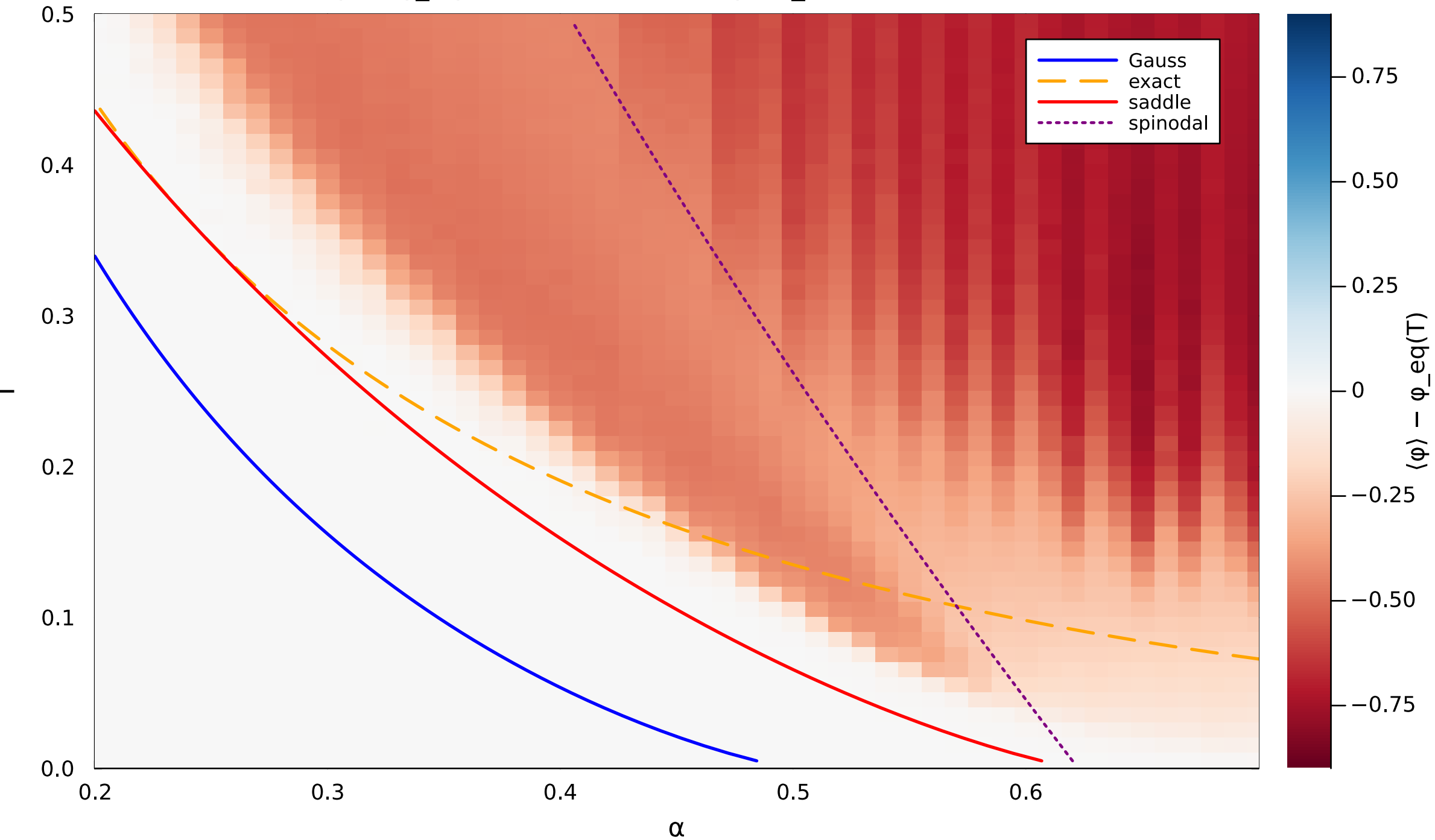
\langle \phi \rangle - \phi_{\text{eq}}(T) , semismart Nramp ( M_{\text{TARGET}} = 4.4\text{e6} )
