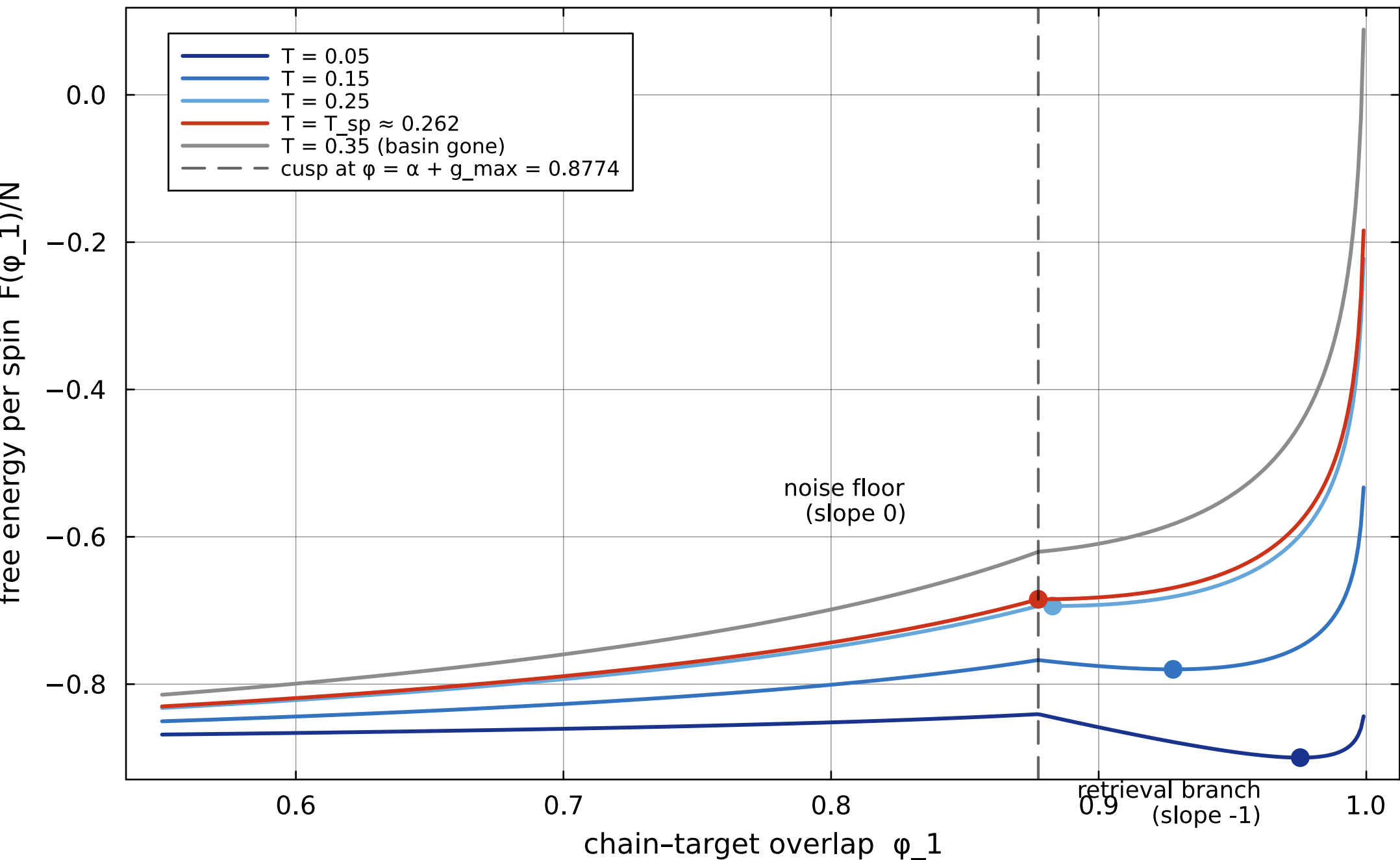
Cusp of the LO free energy ( \alpha = 0.5 , g_{\text{max}} \approx 0.3774 )
