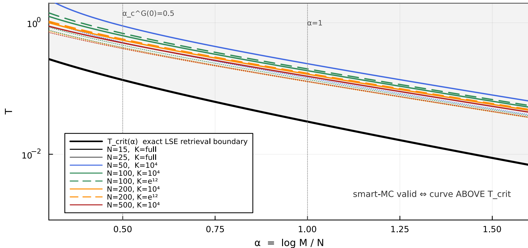
Smart-MC validity window vs. exact LSE retrieval boundary
