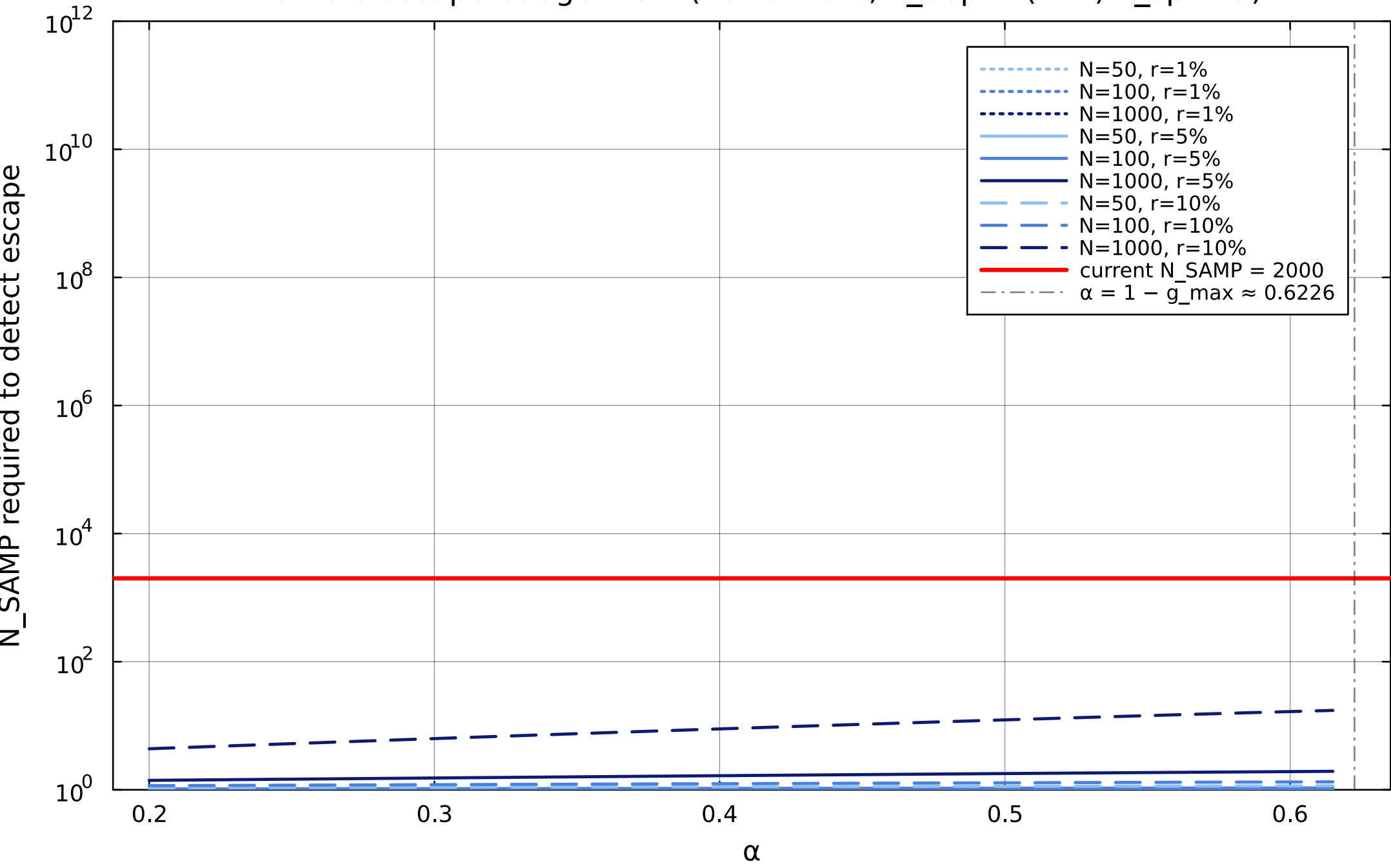
Kramers escape budget vs \alpha (LO formula, T_{\text{dep}} = (1-r) \cdot T_{\text{sp}}^{\text{LO}} )
