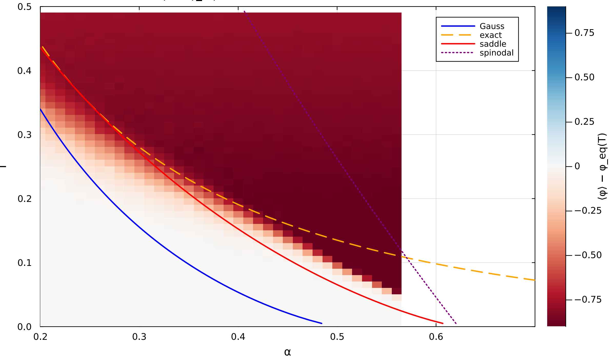
\langle \phi \rangle - \phi_{\text{eq}}(T) , honest MC at N = 25 ( \alpha \leq 0.56 )
