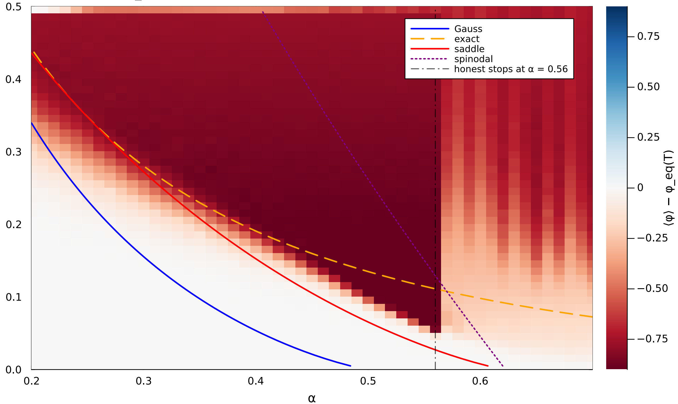
\langle \phi \rangle - \phi_{eq}(T) , honest N=25 overlay on semismart Nramp ( M \approx 4.4e6 )
