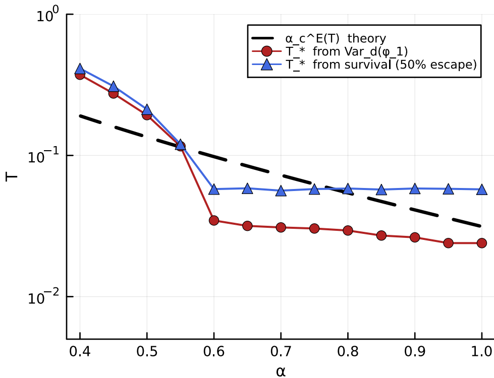
Smart-MC T^*(\alpha) vs theoretical \alpha_c^E(T) \bar{N}=500 K=10000
