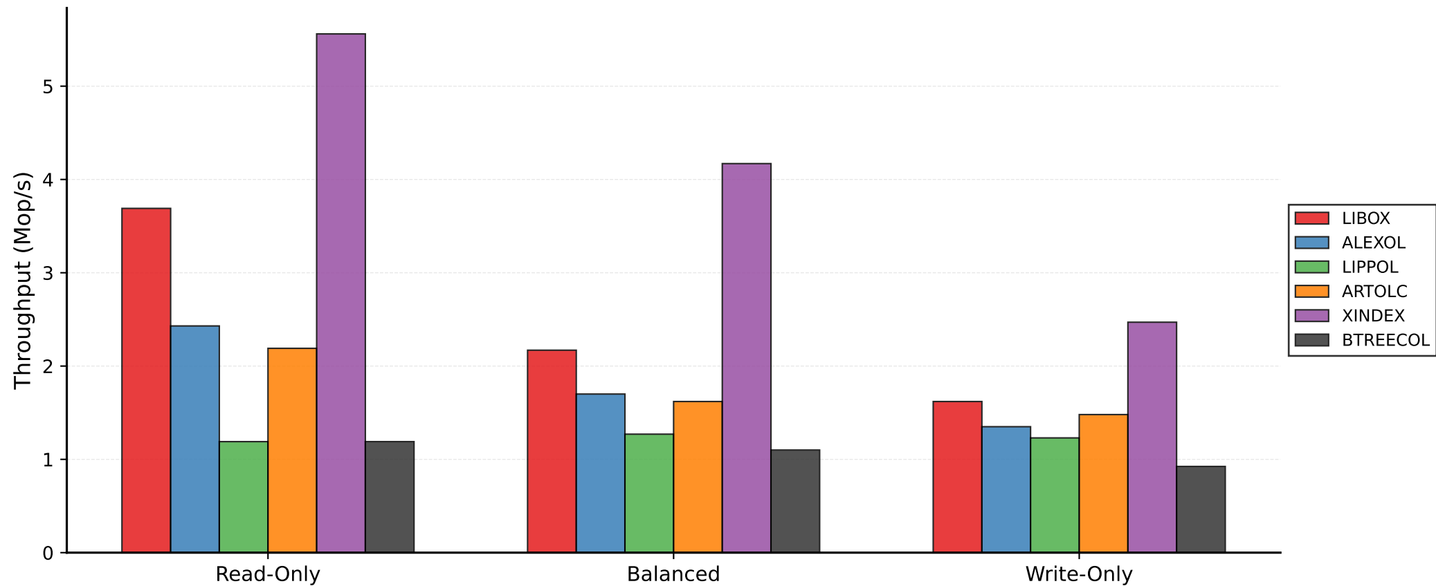
Performance Comparison: Genome
