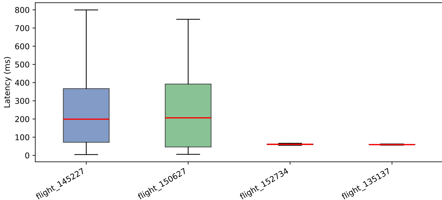
Inference Latency Distribution by Configuration
