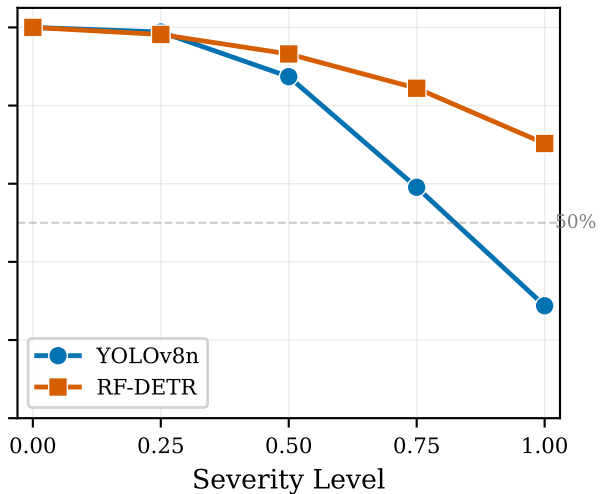
Low Light
