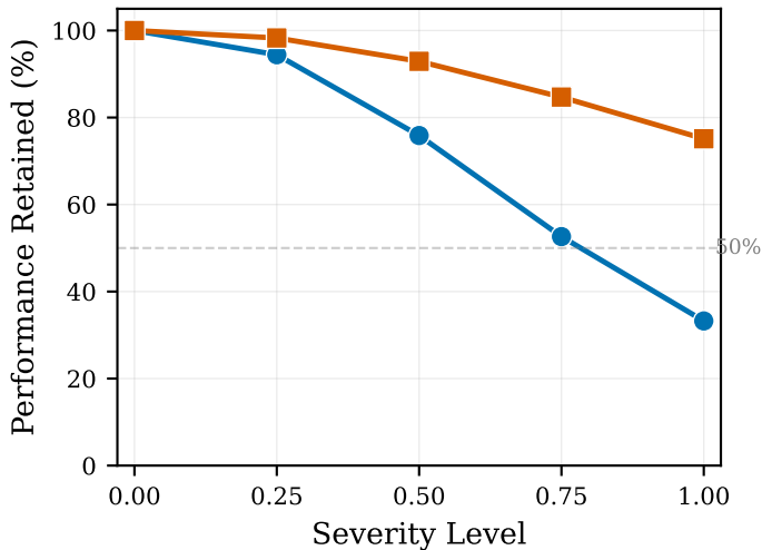
Gaussian Noise
