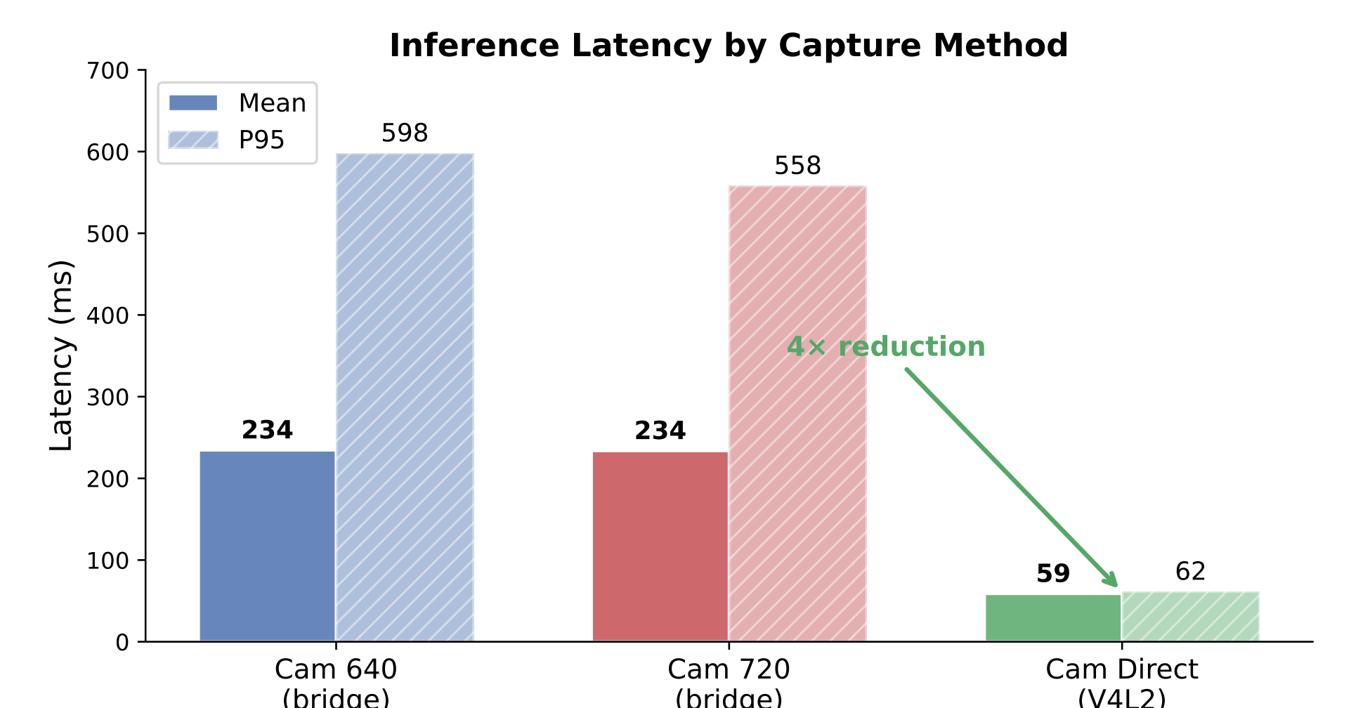
Fig. 4: Mean and P95 inference latency by capture method. V4L2 direct capture eliminates the DDS serialization bottleneck, reducing latency 4 \times .
