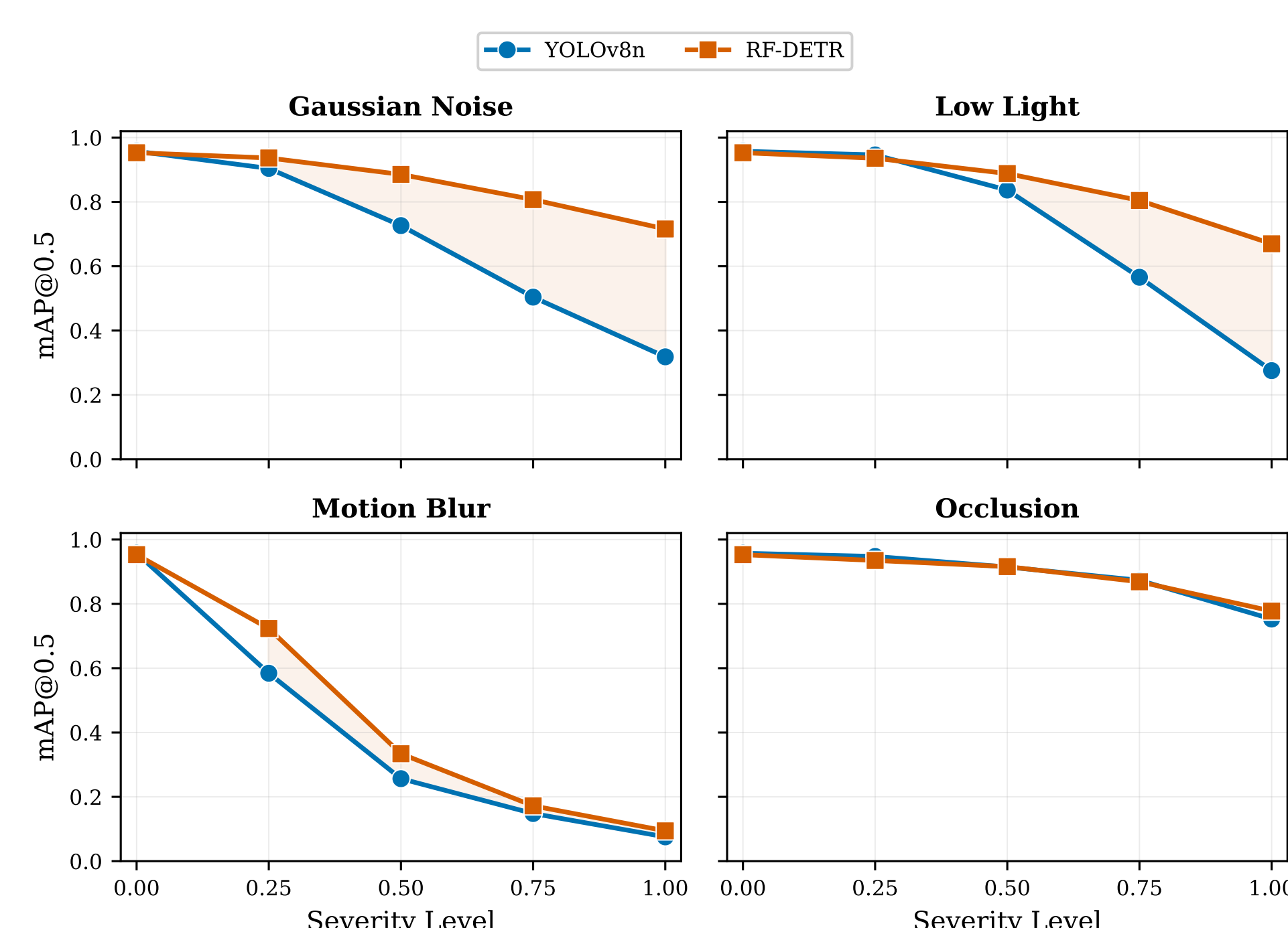
Fig. 2: Detection accuracy (mAP@0.5) under increasing degradation severity. RF-DETR (transformer) maintains substantially higher accuracy than YOLOv8n (CNN) under Gaussian noise and low-light conditions.
