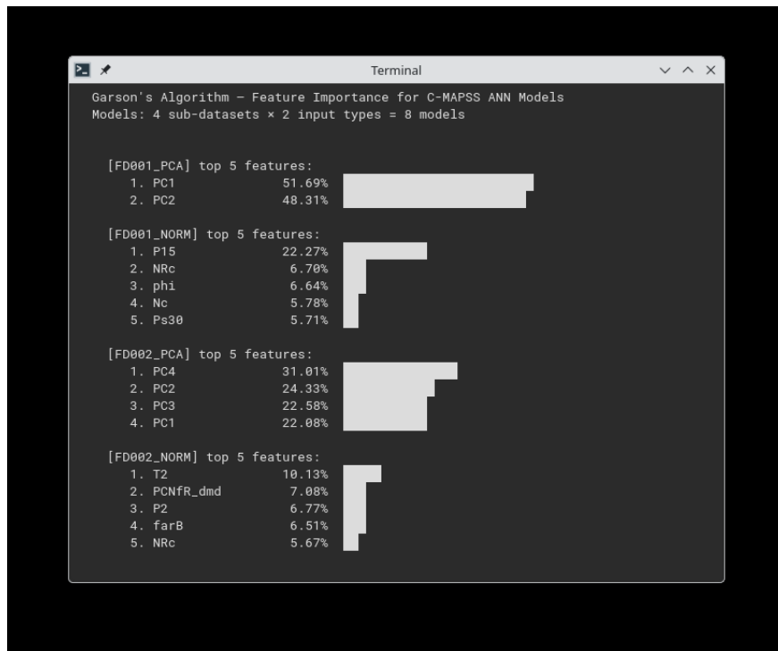
Figure 12: Output terminal algoritma Garson — top 5 fitur FD001 dan FD002
