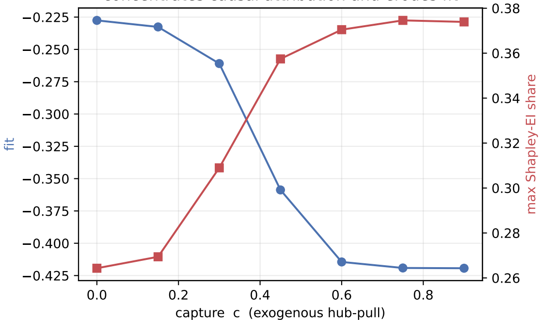
Capture: an independent dial concentrates causal attribution and erodes fit
