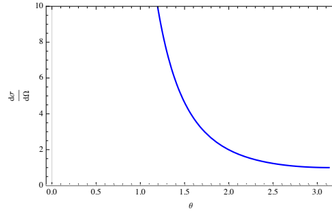
Figure 108: ...and for the Coulomb potential.
