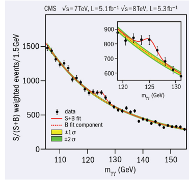
Figure 104: And for the Higgs boson.
