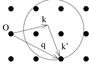
Figure 109: The Ewald sphere.
