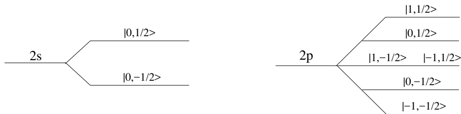
Figure 83: Splitting of the 2s and 2p energy levels in a magnetic field. The quantum numbers |m_l, m_s\rangle are shown.
