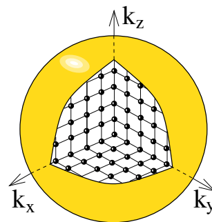
Figure 35: The Fermi surface
