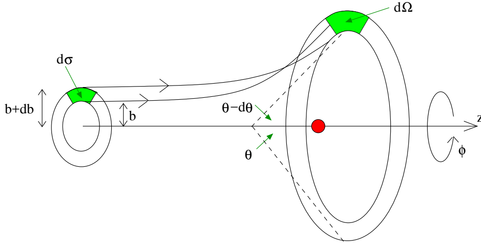
Figure 97: What becomes of an infinitesimal cross-sectional area after scattering.
