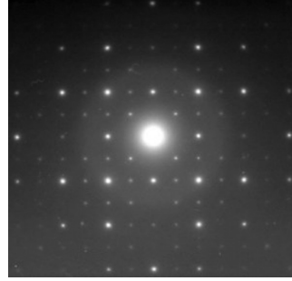
Figure 110: Salt.
