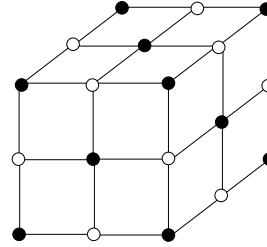
Figure 115: The reciprocal as a cubic lattice minus a basis.
