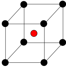
Figure 114: A BCC lattice as cubic lattice + basis.
