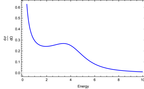
Figure 102: ...and with \Gamma^2 = 15
