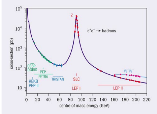
Figure 103: The cross-section for the Z-boson.
