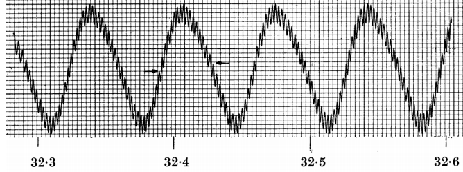
Figure 54: dHvA oscillations for gold. The horizontal axis is B , plotted in kG .
