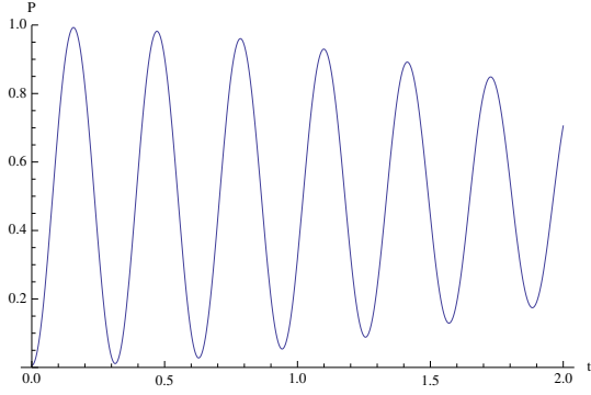
Figure 84: Rabi Oscillations at short times...
