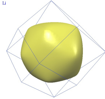
Figure 37: Lithium.
