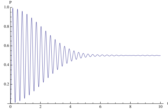
Figure 85: ...and their decay at longer times.
