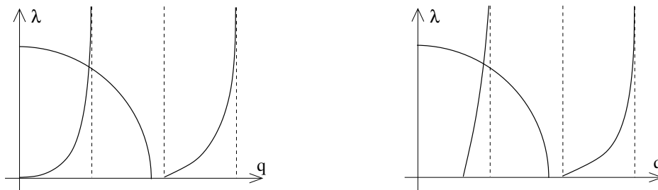
Figure 93: Bound state of even parity always exist, since the two equations shown on the left always have a solution with \lambda, q > 0 . Bound states of odd parity, shown on the right, exist if the potential is deep enough.
