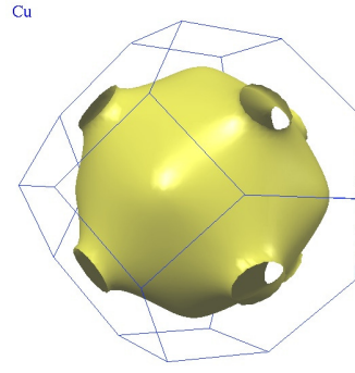
Figure 38: Copper.
