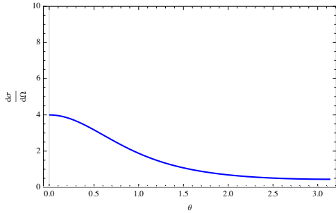
Figure 107: The cross-section for the Yukawa potential...
