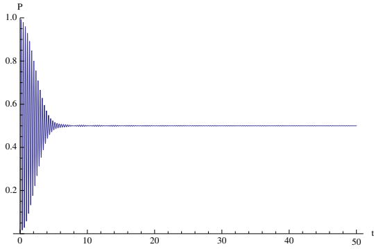
Figure 86: Once decayed, they stay decayed...
