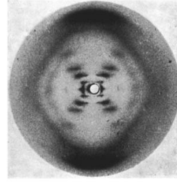
Figure 112: DNA, Photograph 51.
