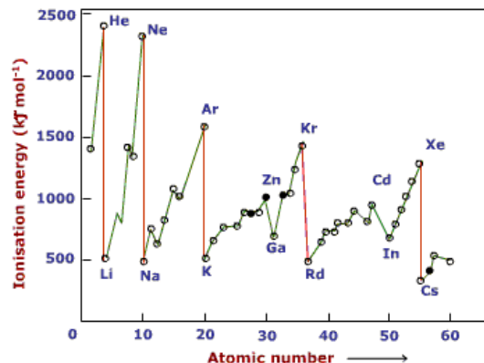
Figure 81: Ionization data again.
