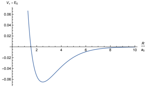
Figure 73: The potential for \Psi_+
