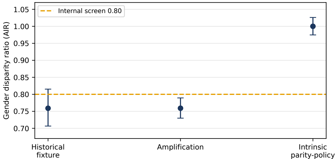
Single-run branch characterization (95% conditional intervals)
