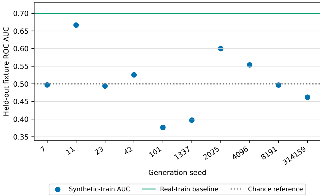
TSTR utility varies materially across generation seeds
