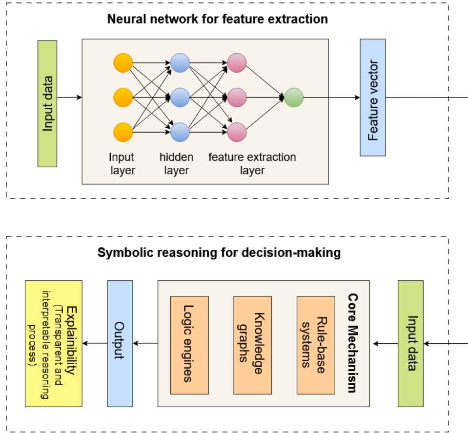
Fig. 3. Hybrid model architecture integrating neural networks for feature extraction and symbolic reasoning for decision-making.
