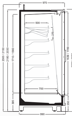
LION V2 PGD/100/220-205
