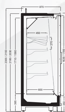
LION V2 PGD/90/220-205
