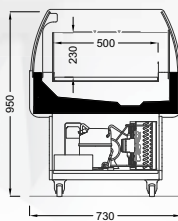
SPIDER 800/1850
