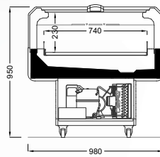
SPIDER SLD 800/1050
