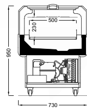
SPIDER SLD 800/1850
