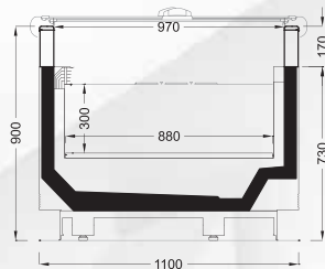
DOLPHIN IS/G20/110 SLD
