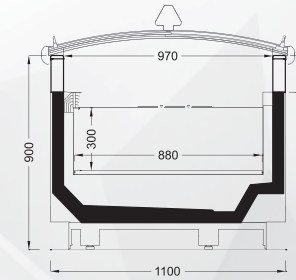
DOLPHIN IS/G20/110 PUSH-PULL SLD
