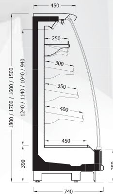
FALCON MT/75/180-170-160-150 SLD SG
