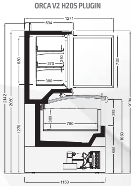
With Push-Pull Curved Glass Lids For Bottom
