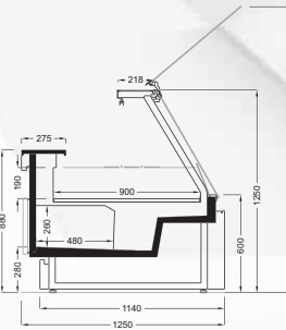
KANGAROO V1 900 WFG/CB
