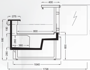
KANGAROO V1 800 WFG/CB
