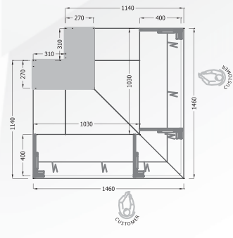
TIGER 800 FG/CB-OF/OC 90°
