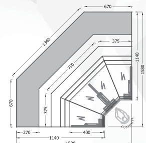
TIGER 800 FG/CB-OF/IC 90°
