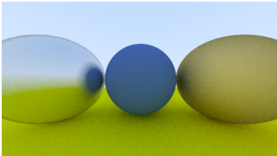
Image 14: Fuzzed metal
