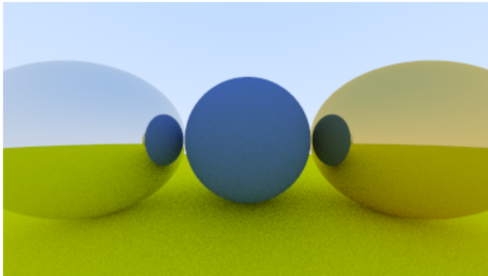
Image 13: Shiny metal
