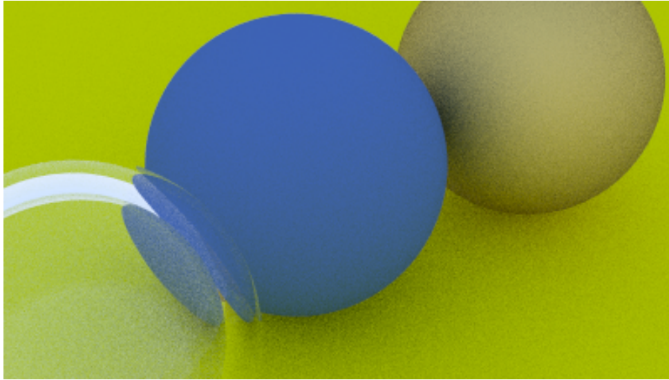
Image 21: Zooming in
