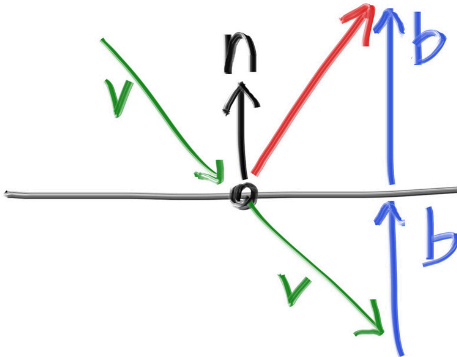
Figure 15: Ray reflection
