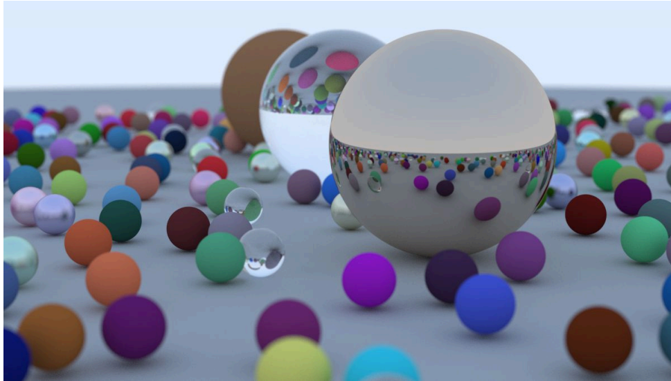
Image 23: Final scene
