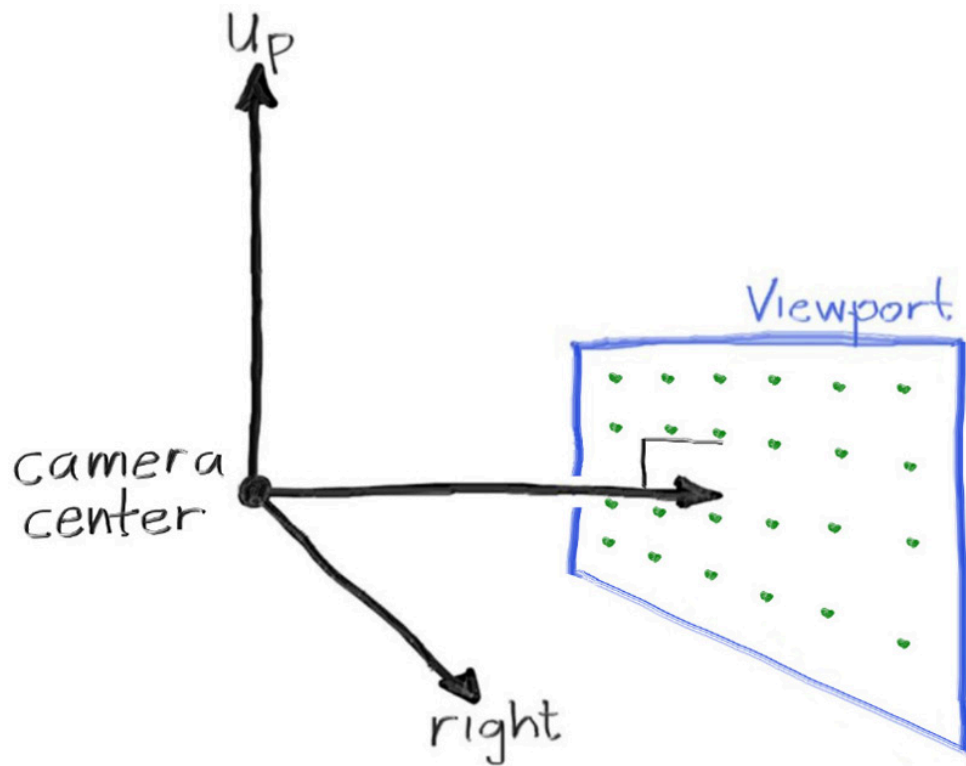
Figure 3: Camera geometry
