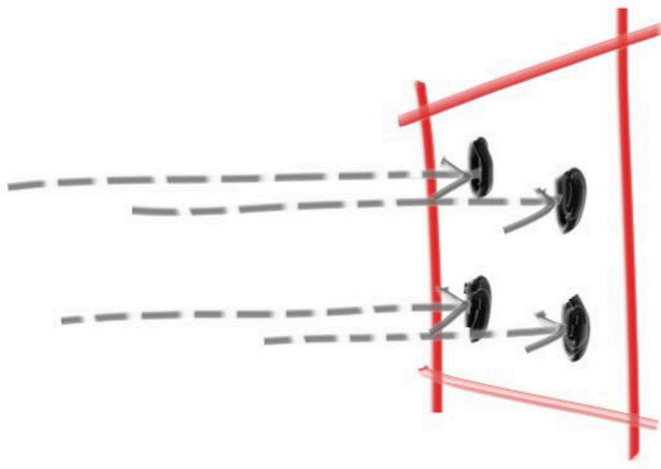
Figure 8: Pixel samples
