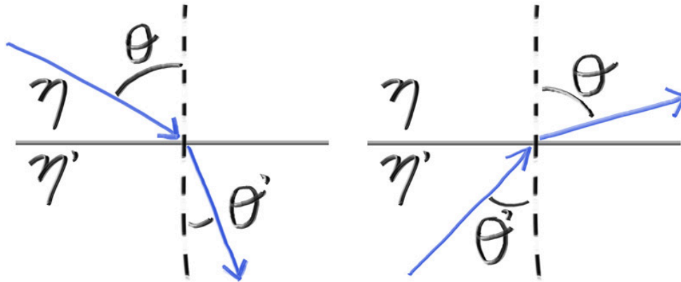
Figure 17: Ray refraction
