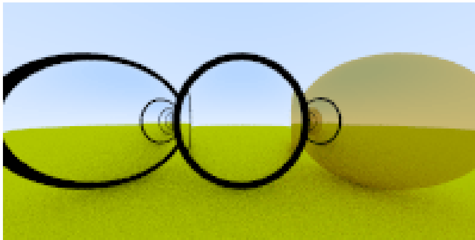
Image 15: Glass first
