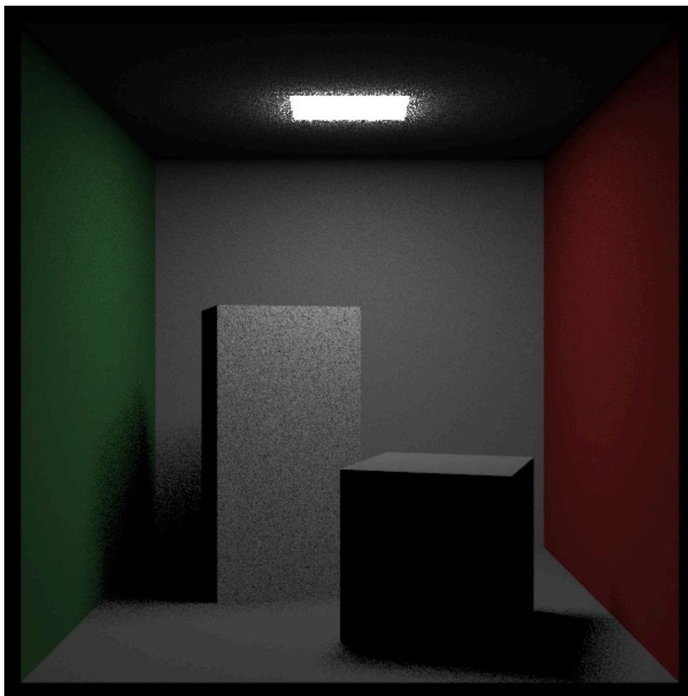
Image 7: Cornell box, sampling only the light, 10 samples per pixel
