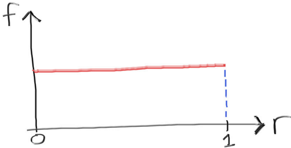
Figure 5: A uniform distribution
