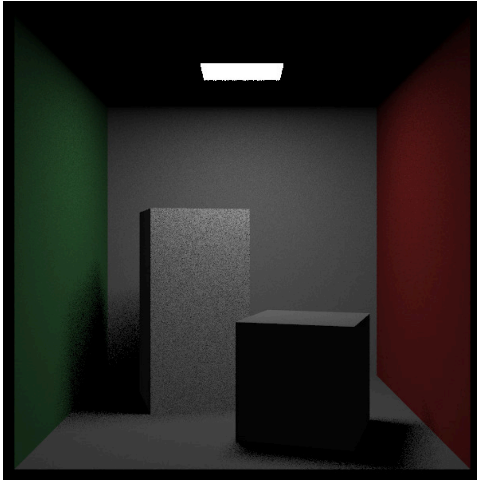
Image 10: Cornell box, sampling a hittable light, 10 samples per pixel
