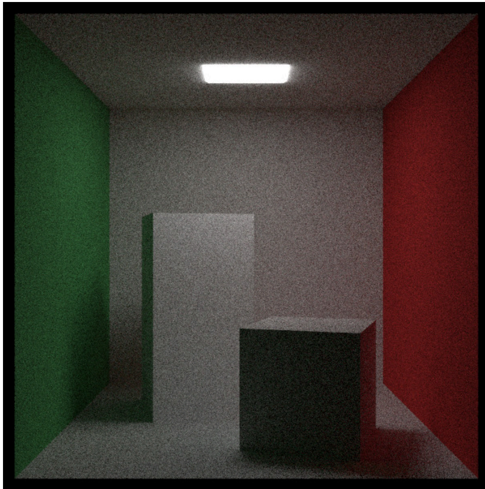
Image 5: Cornell box, with uniform hemispherical sampling
