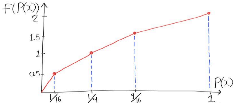
Figure 8: Approximating the nonuniform f()
