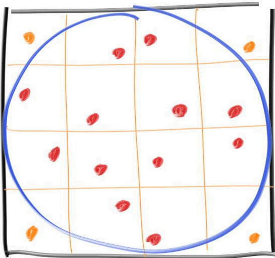
Figure 2: Sampling areas with jittered points
