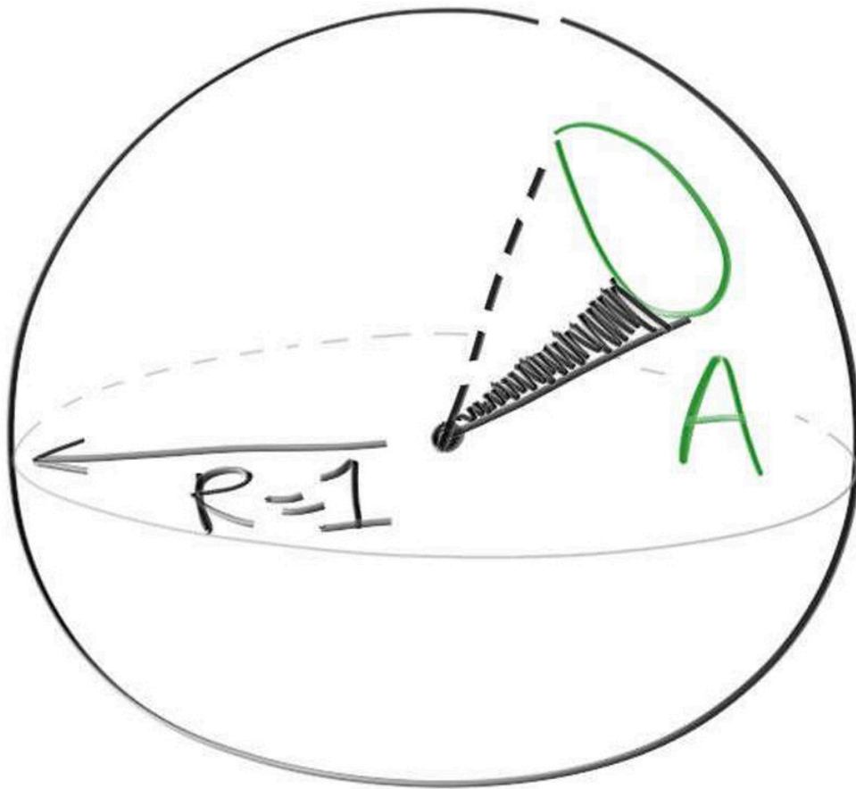
Figure 9: Solid angle / projected area of a sphere
