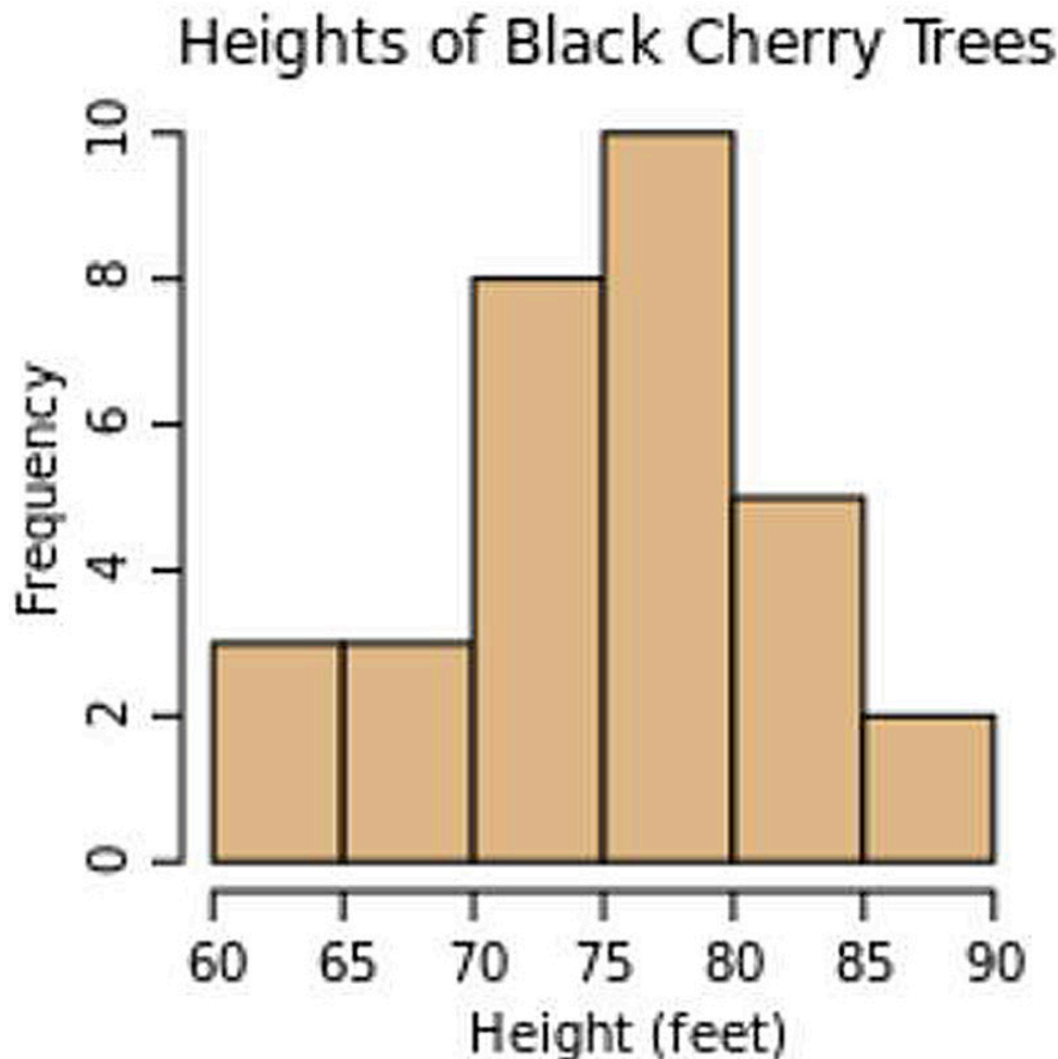
Figure 3: Histogram example
