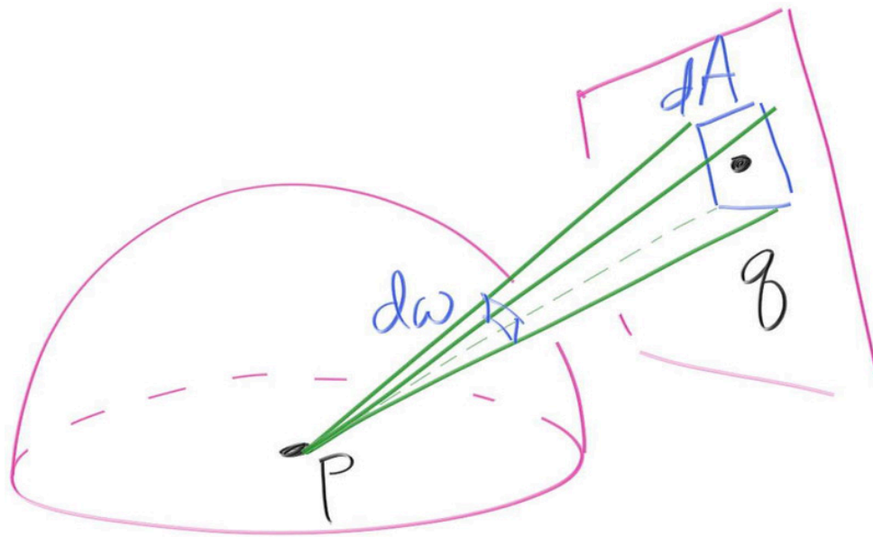
Figure 11: Projection of light shape onto PDF
