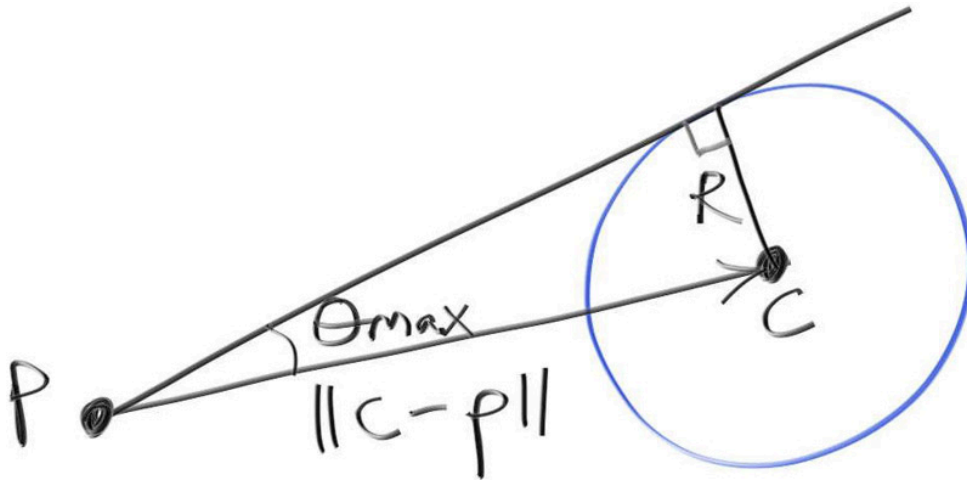
Figure 12: A sphere-enclosing cone
