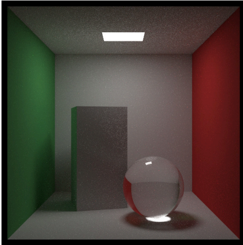
Image 14: Cornell box using a mixture of glass & light PDFs
