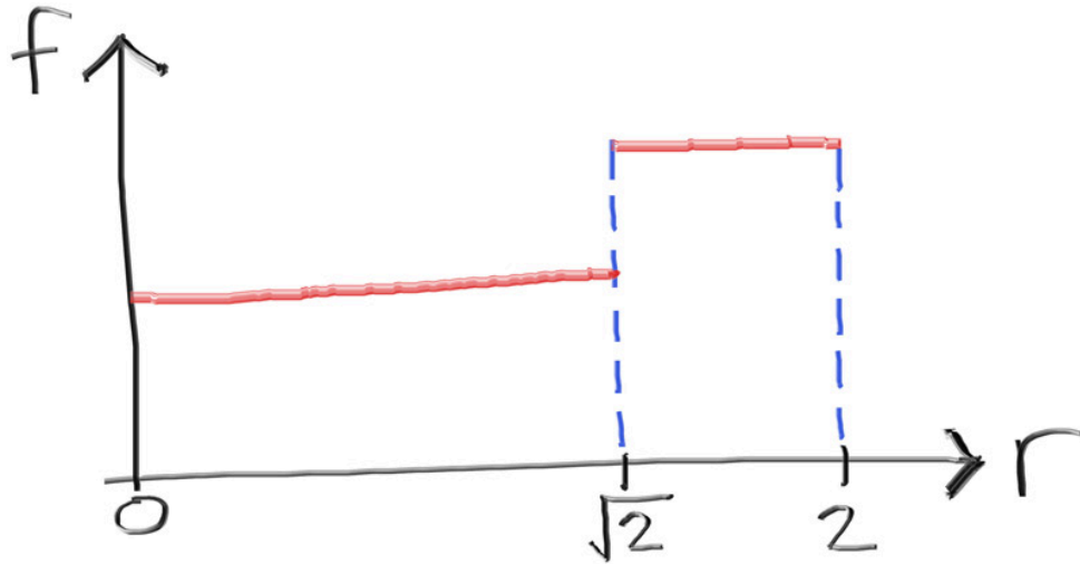
Figure 6: A nonuniform distribution for r/2
