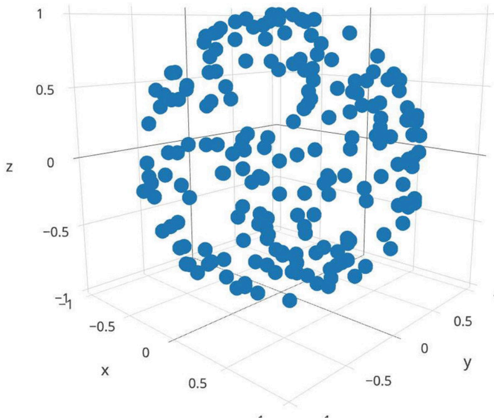
Figure 10: Random points on the unit sphere
