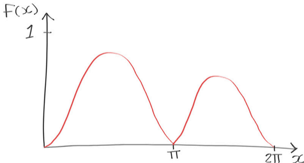
Figure 7: A function that we don't want to solve analytically
