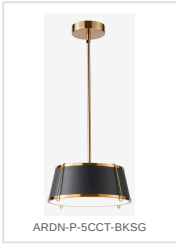
ARDN-P-5CCT-BKSG
