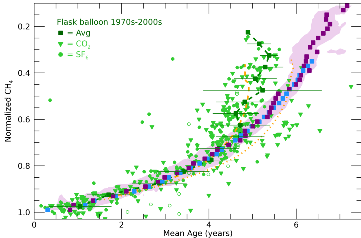
a Mean Age vs. CH 4
