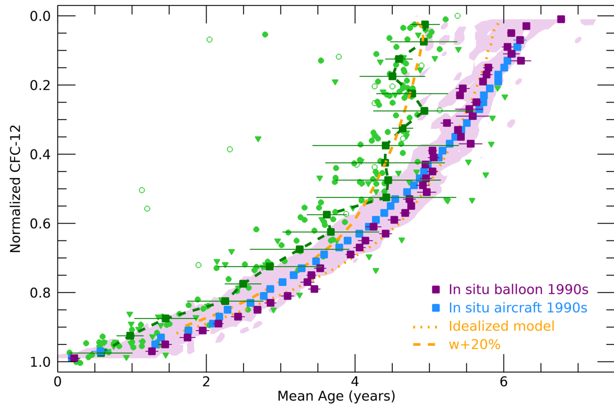
b Mean Age vs. CFC-12
