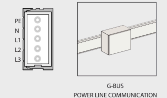
G-BUS POWER LINE COMMUNICATION
