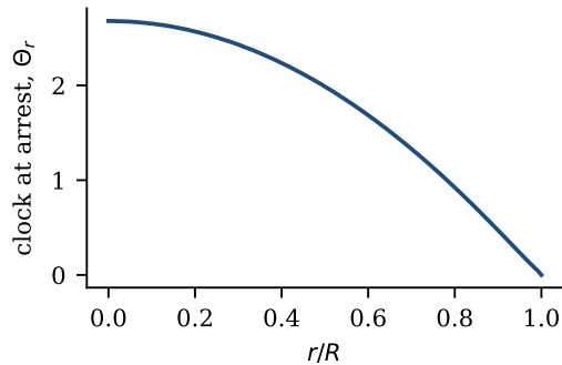
(b) Lemma 1: \Theta_r monotone in r
