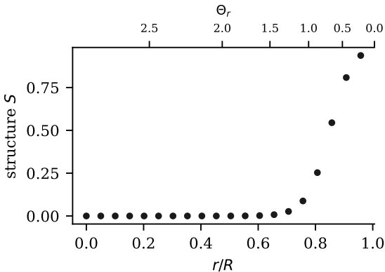
(c) Proposition 1: the same data on two axes
