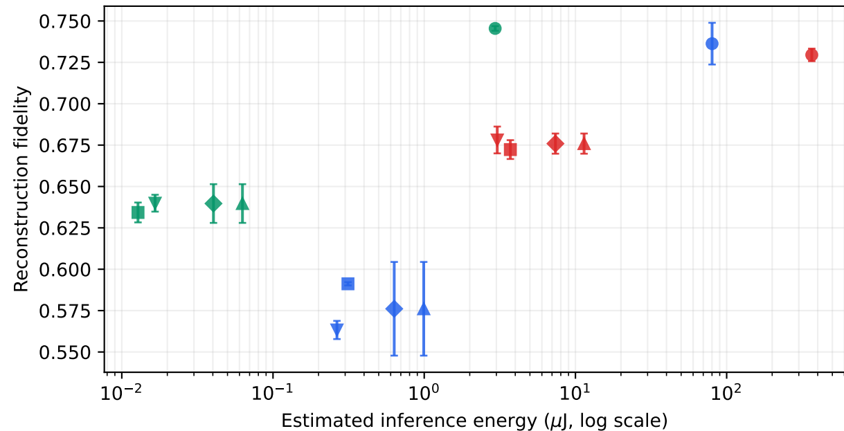
Bures Mixed
