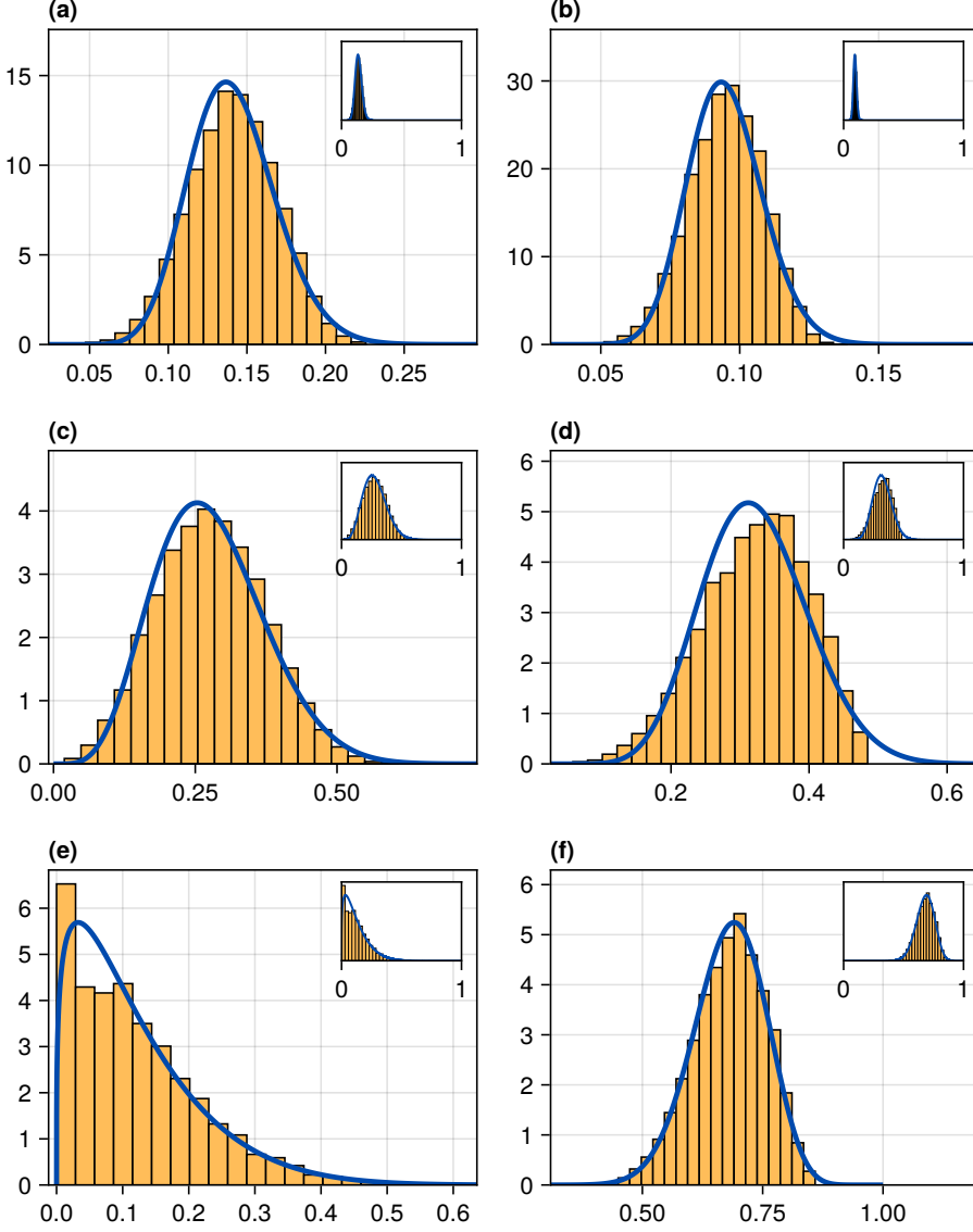
Figure 3: Six learning simulation experiments. In each experiment, 10,000 learners were simulated to equilibrium with randomly drawn parameters (see Table 3). The equilibrium distribution of W_1 , the weight on G_1 (yellow histogram), is well approximated by a Beta distribution (blue curves indicating the probability density function) found by moment matching. Insets scale each facet to the entire range of possible values of W_1 , the interval [0, 1] .
