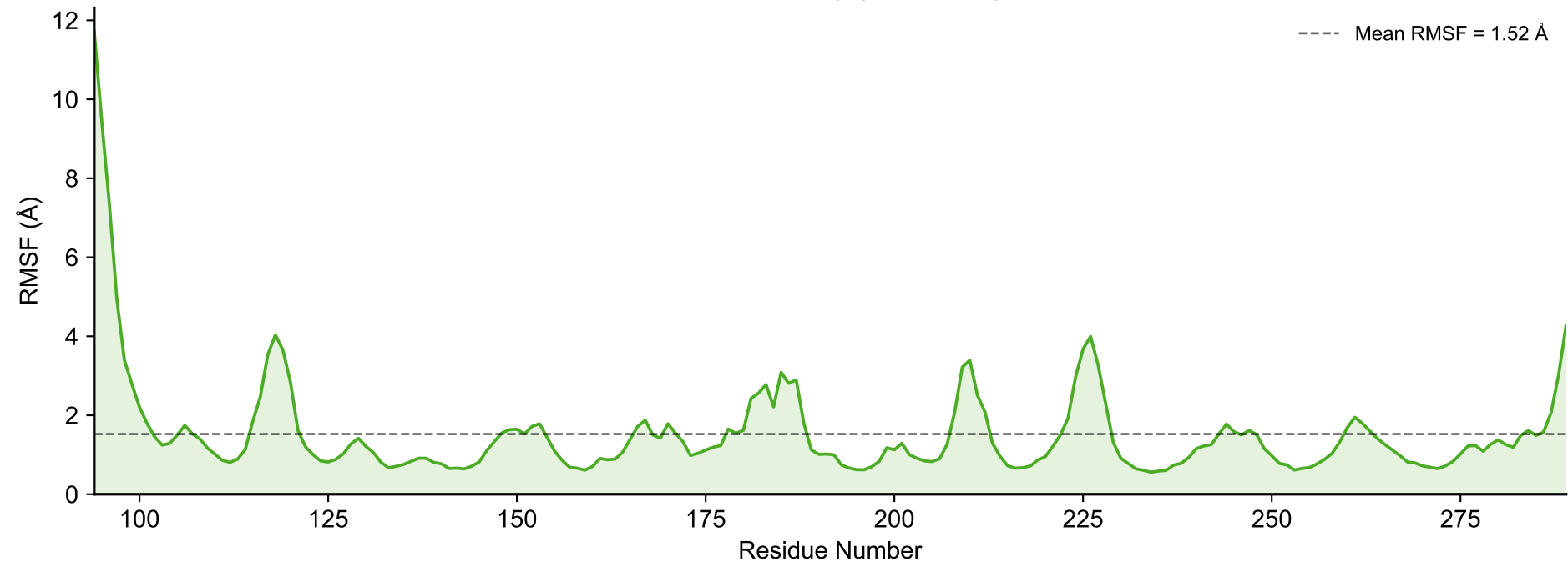
Per-Residue Flexibility (Backbone) — 1 \mu s
