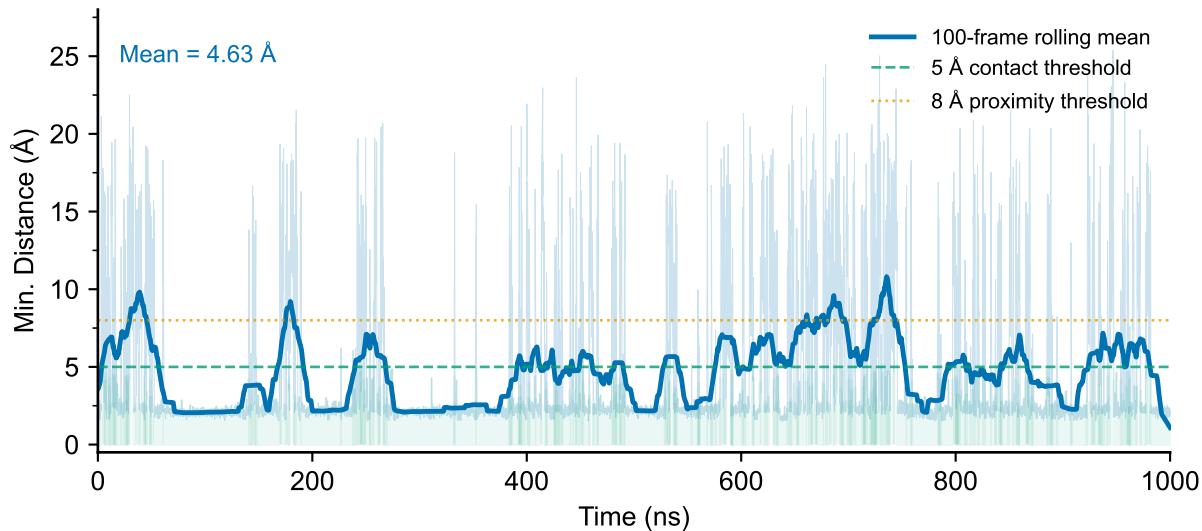
(A) Protein–Carvacrol Minimum Distance — 1 \mu s MD
