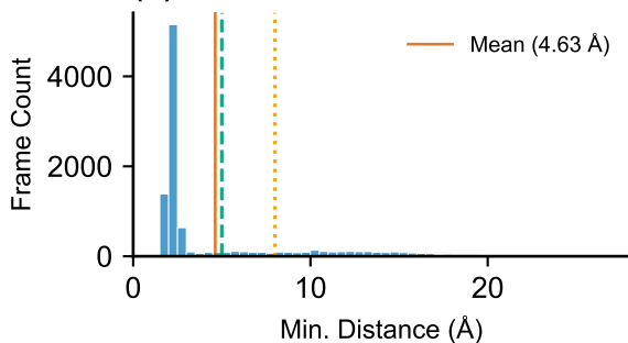
(B) Distance Distribution
