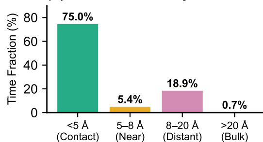
(C) Contact Zone Analysis
