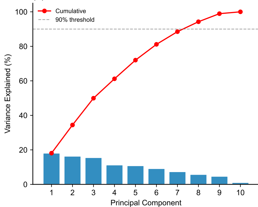
(B) Scree Plot
