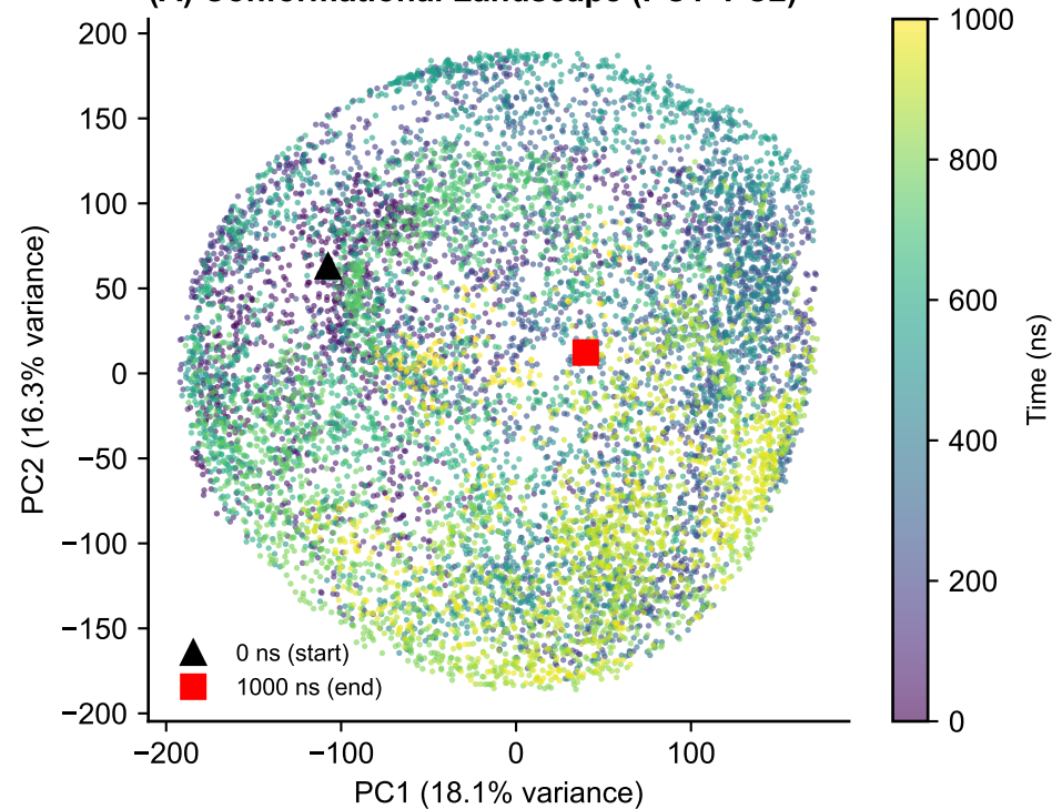
(A) Conformational Landscape (PC1–PC2)
