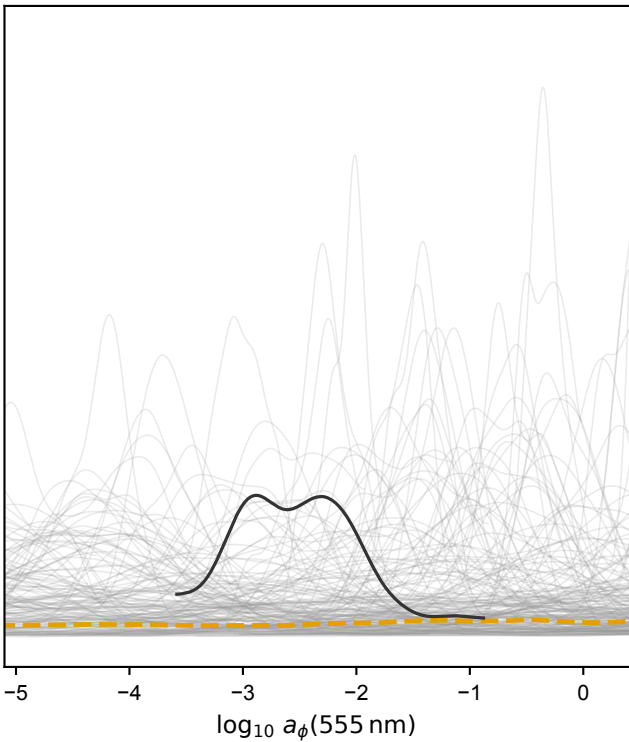
Prior predictive
