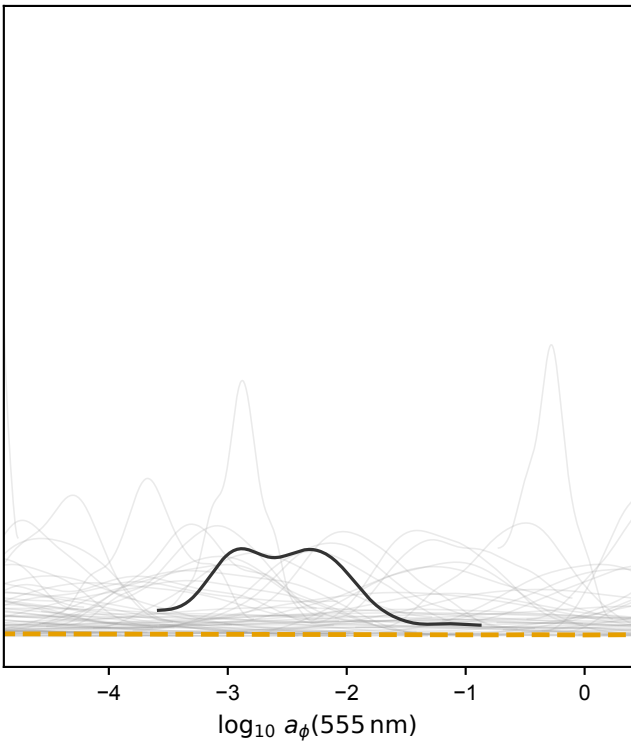
Prior predictive
