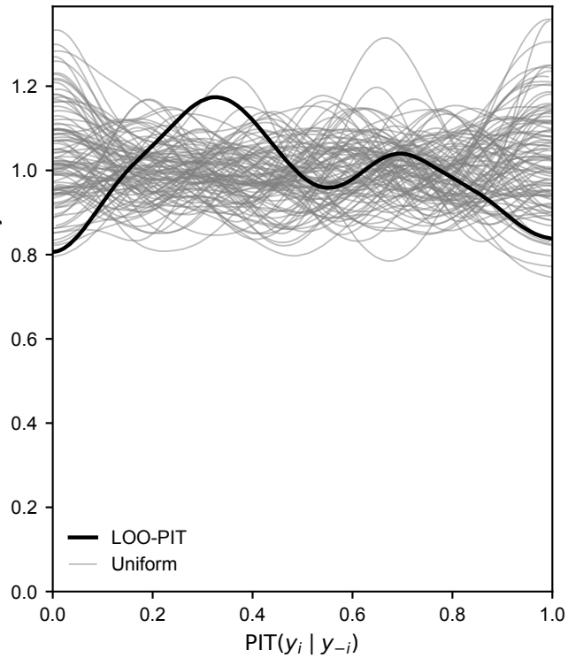
LOO-PIT
