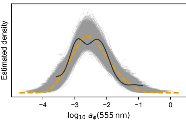
PPC ( \lambda = 555 nm)
