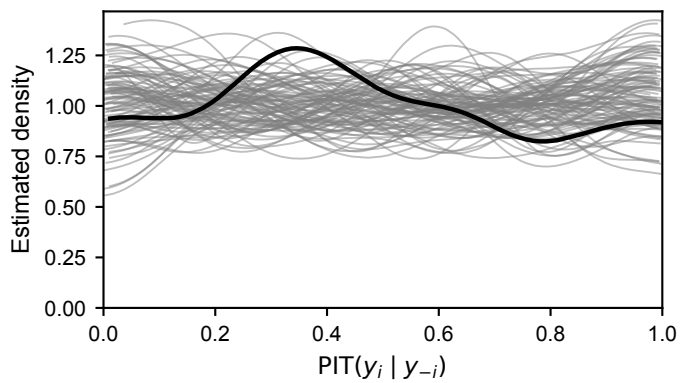
LOO-PIT
