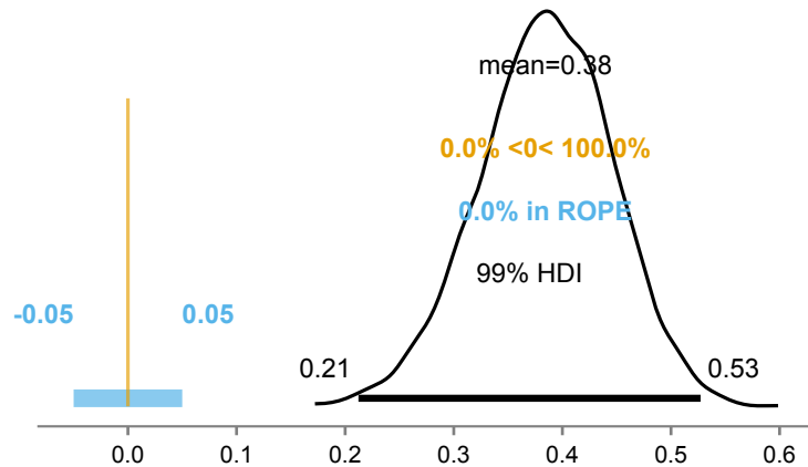
corr(resid_aph555, resid_aph670)
