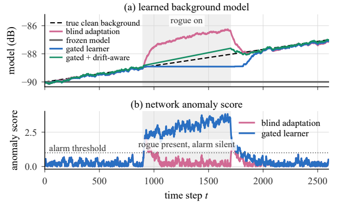
Fig. 1. An 800-sample rogue dwell, i.e., a continuous interval during which the rogue transmitter remains active. The blindly adapting learner gradually incorporates the rogue into its background model, causing the anomaly score to fall below the alarm threshold while the rogue remains present. Gating prevents this adaptation and keeps the alarm active, but the frozen background estimate becomes stale as the environment drifts. The drift-aware variant continues to track the background while the gate is closed.
