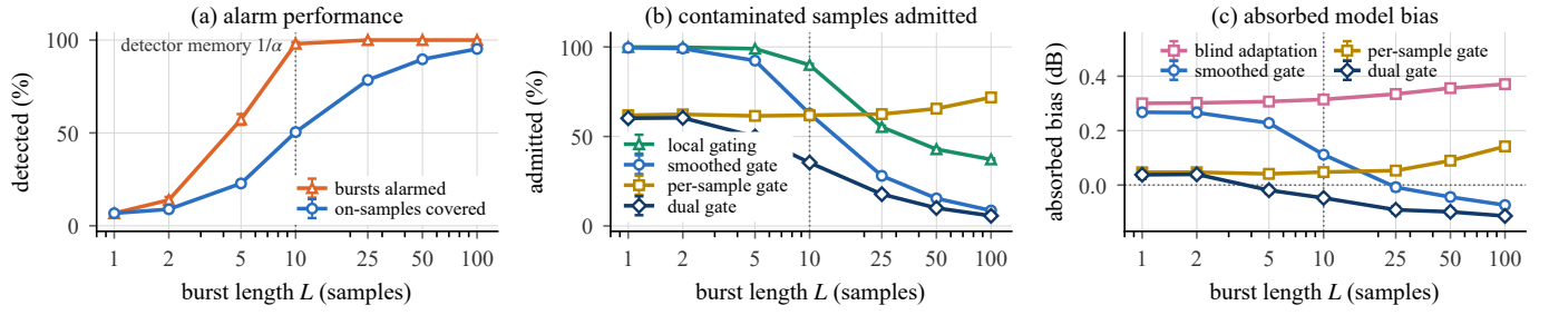
Fig. 3. Fragmentation of a fixed transmit budget, 100 contaminated samples of a 400-sample window with all reachable receivers hit together, 20 seeds, \pm 1 SEM. Only the burst length L varies, and the per-sample clean-reference detection rate stays at 44 to 46%. (a) Alarm performance collapses below the detector memory 1/\alpha = 10 , counted per burst (upper) and per contaminated sample (lower). (b) Smoothed gates admit nearly everything at small L , the per-sample gate is timing invariant, and the dual gate admits the fewest at every L . (c) The blind learner’s absorbed bias barely moves, while the dual gate never absorbs more than +0.04 dB, at the price of a small stale-model lag at long bursts.
