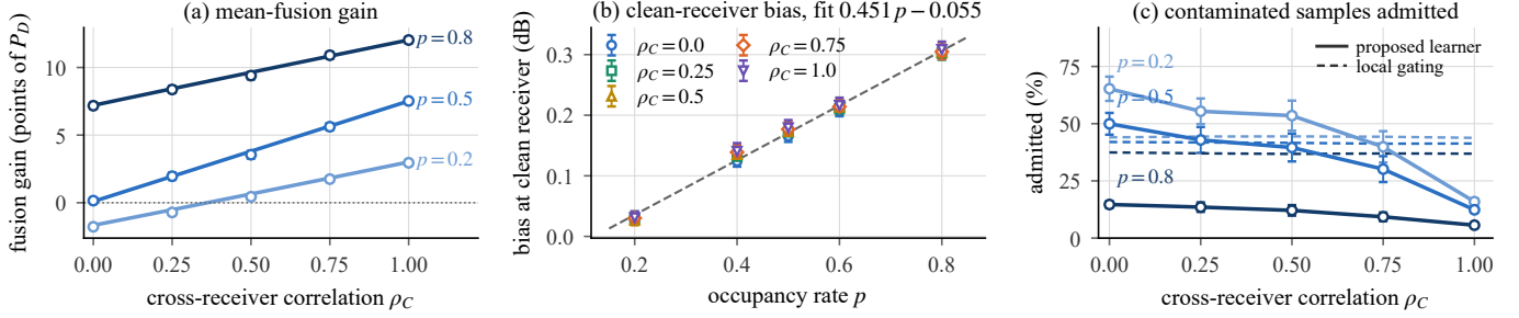
Fig. 2. Behavior over the occupancy rate and correlation plane. (a) Mean-fusion gain over the strongest single receiver. Lines show exact theory and points show simulation with 200 seeds and \pm 1 SEM bars. (b) Bias propagated into the clean receiver under unprotected mixing. All five correlation levels land on one line in the rate, as Proposition 1 requires. (c) Contaminated samples admitted. The proposed learner, solid, exceeds local gating, dashed, at low rates when \rho_C = 0 and crosses below it as p and \rho_C grow. Panels (b) and (c) use 20 seeds per cell.
