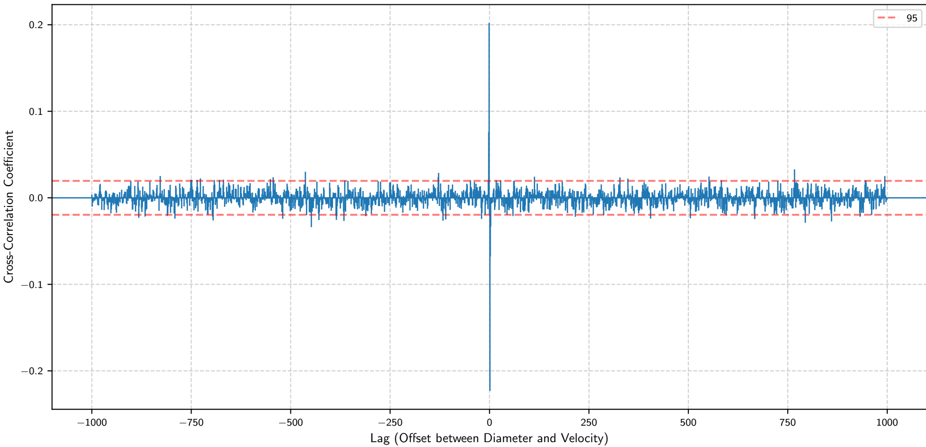
Cross-Correlation between Diameter and Velocity
