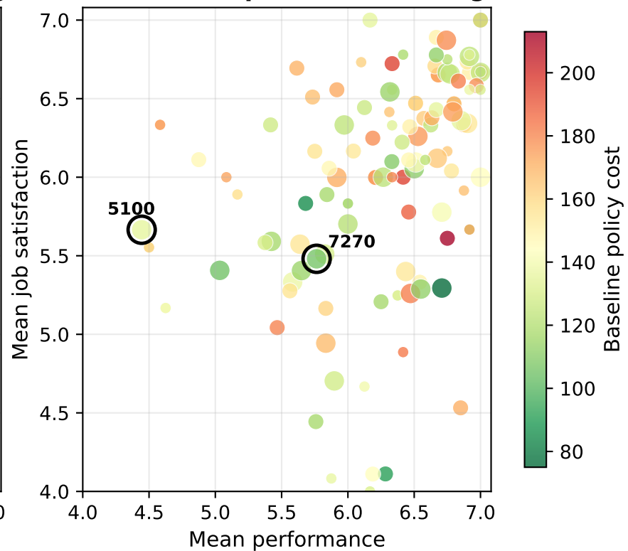
Decision tree predictions (design)
