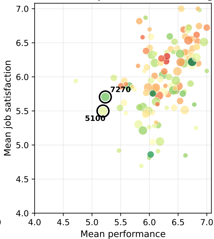
Mixed model predictions (redesign)
