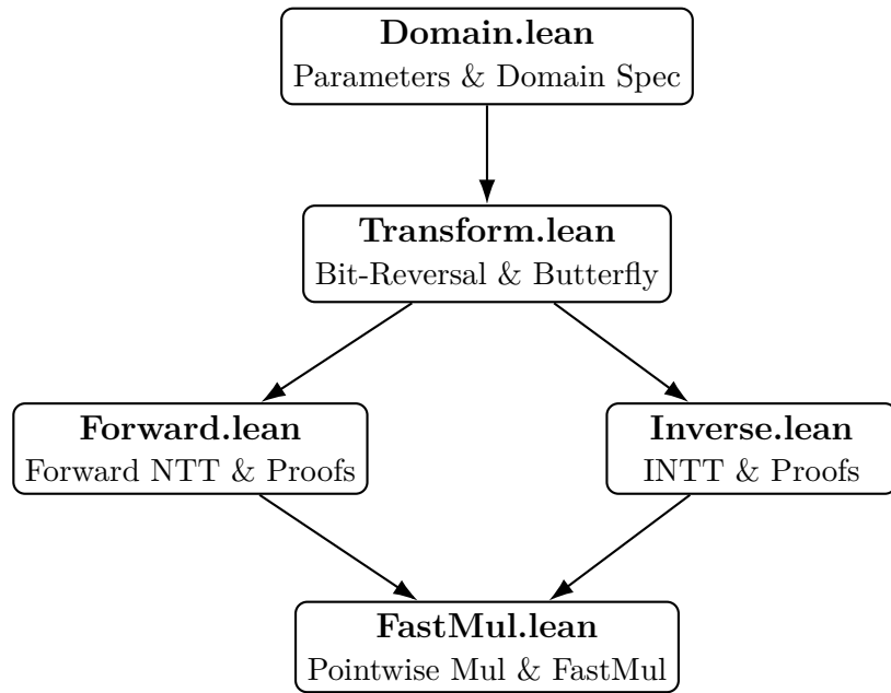
Figure 6.2: Module Dependency Graph for the NTT Pipeline
