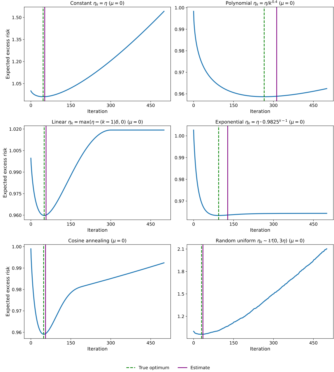
Figure 2: Bayes excess risk trajectories for the unregularized least squares problem ( \mu = 0 ) with the MNIST dataset. The six panels compare different learning rate schedules. The green dashed line shows the empirical optimal stopping time, and the purple line shows our estimated stopping time from (30).
