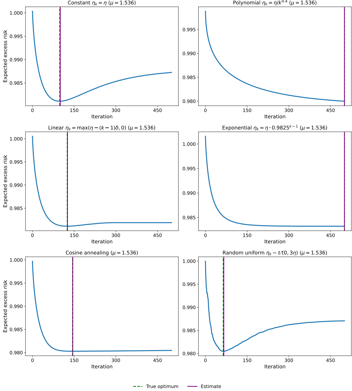
Figure 6: Bayes excess risk trajectories for the ridge-regularized least squares problem with \mu = 1.536 with the CIFAR10 dataset. This corresponds to \mu = \mu^*/2 , where \mu^* = 3.072 is the optimal ridge parameter. The six panels compare different learning rate schedules. The green dashed line shows the empirical optimal stopping time, and the purple line shows our estimated stopping time from (30).
