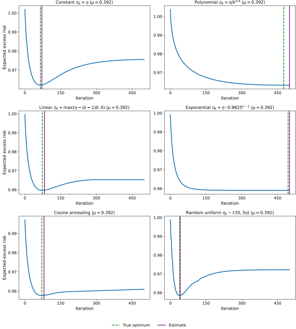
Figure 3: Bayes excess risk trajectories for the ridge-regularized least squares problem with \mu = 0.392 with the MNIST dataset. This corresponds to \mu = \mu^*/2 , where \mu^* = 0.784 is the optimal ridge parameter. The six panels compare different learning rate schedules. The green dashed line shows the empirical optimal stopping time, and the purple line shows our estimated stopping time from (30).
