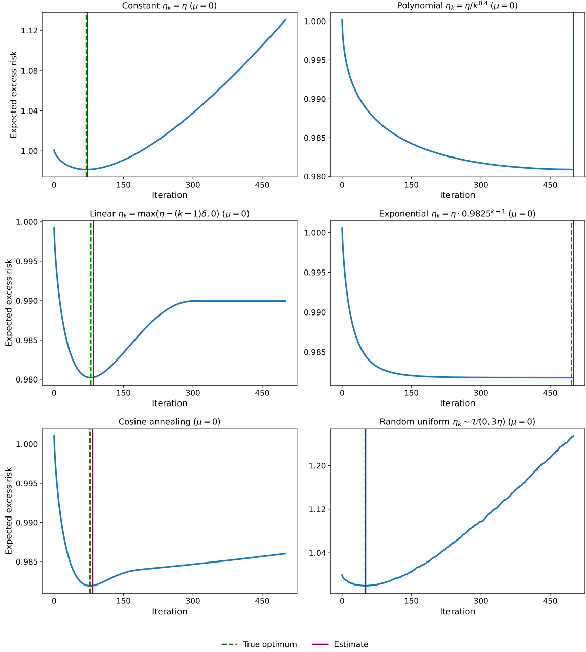
Figure 5: Bayes excess risk trajectories for the unregularized least squares problem ( \mu = 0 ) with the CIFAR10 dataset. The six panels compare different learning rate schedules. The green dashed line shows the empirical optimal stopping time, and the purple line shows our estimated stopping time from (30).
