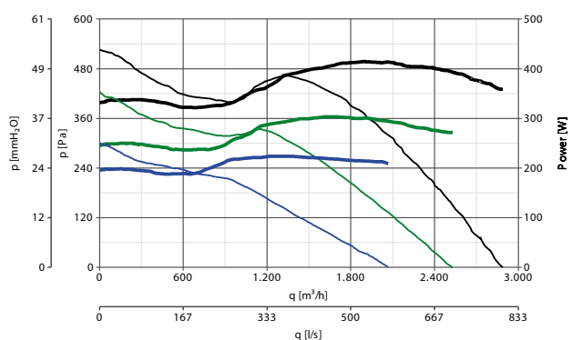
LINEO 315 QUIET
