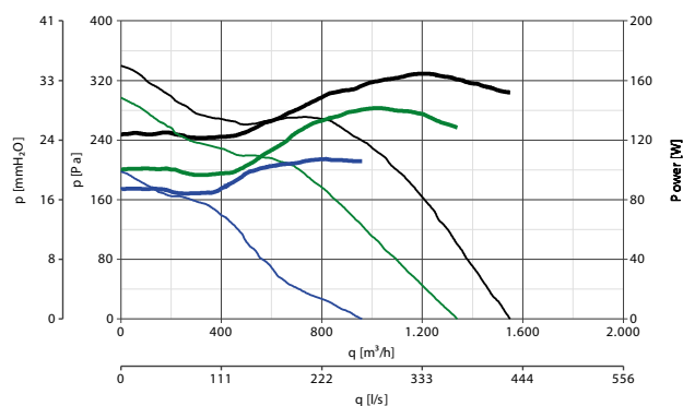
LINEO 250 QUIET
