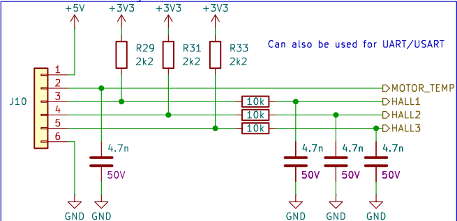
Hall connector and filtering
