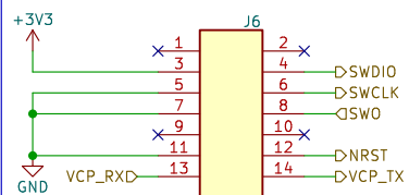
ST-Link V3 MINIE CONNECTOR (STDC14)
