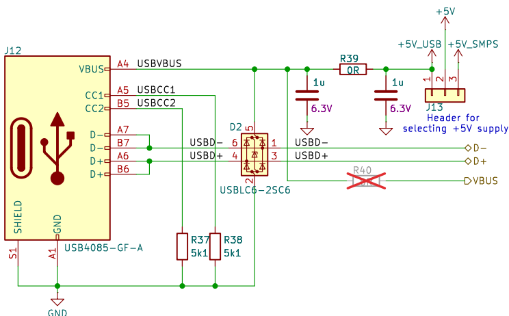
USB-C Connector
