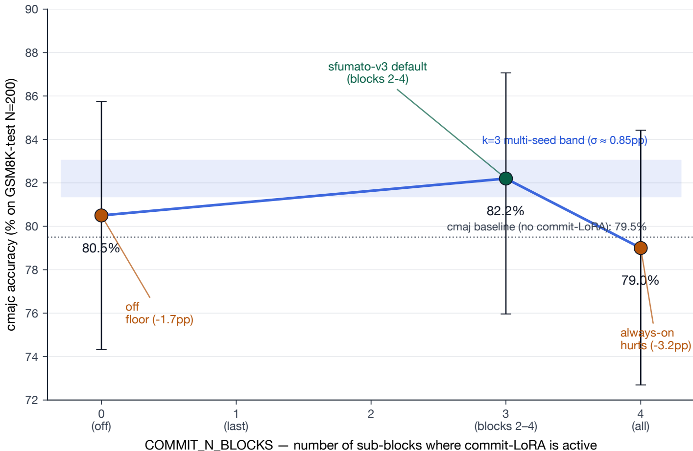
Commit-LoRA timing: schedule-toggle peaks at k=3, drops on either side
