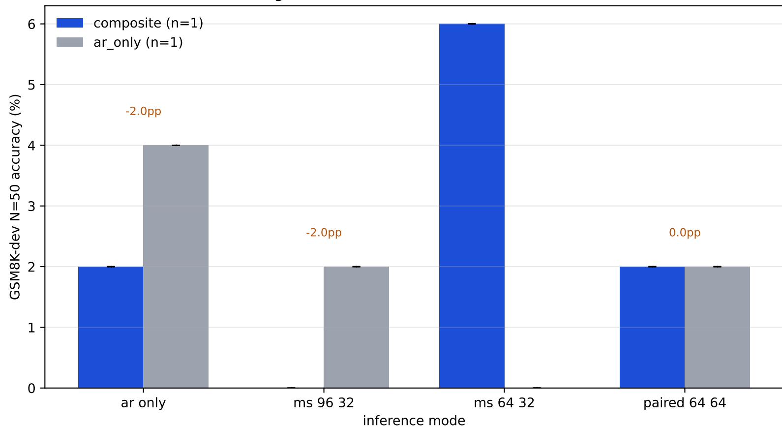
Mode-switching inference lift at 200M-3k (E3a fresh seeds, n=1)
